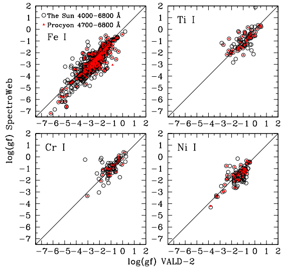
Figure 4. Same as Fig. 1 shown for neutral lines of Fe, Ti, Ni, and Cr ( clockwise ). More neutral lines of Fe, covering a broader range of \log(gf) -values, are selected in the optical spectrum for detailed spectral synthesis compared to Ti, Ni, and Cr.
