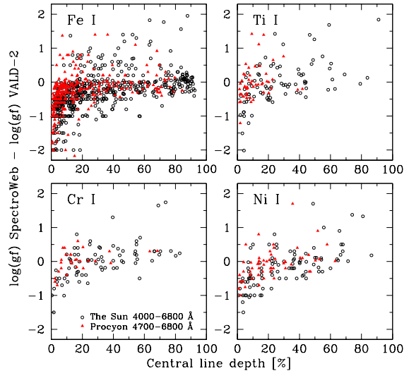
Figure 5. Differences between \log(gf) -values measured in SpectroWeb and offered in VALD compared to the normalized central depth computed for neutral lines of four iron-group elements in Fig. 4. The \log(gf) -values of weak lines are systematically over-estimated in VALD.
